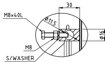
DETAIL "A" (EARTH TERMINAL) (S = 1:4)
